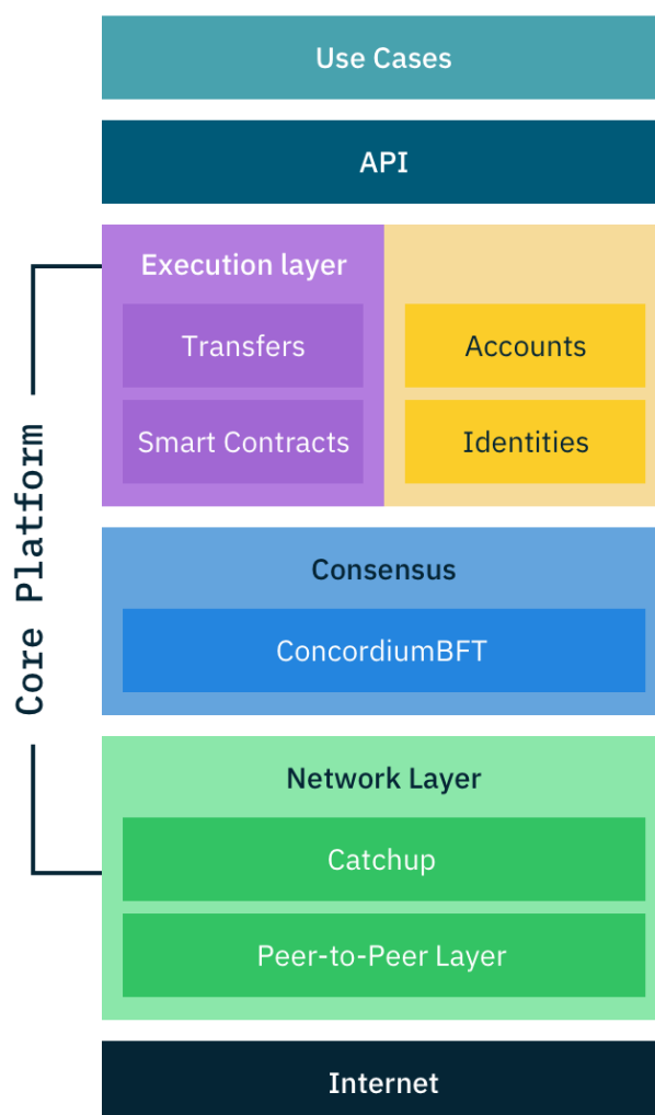
Figure 1: Overview of the Concordium stack.
